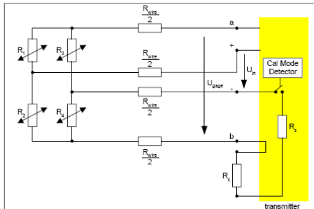
Figure 1- Wheatstone bridge
