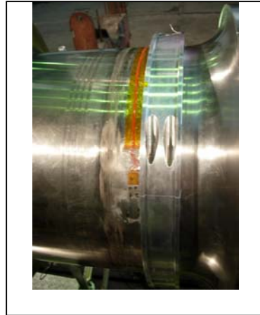
Image 1- Rotating coil and 2 strain gages installed
