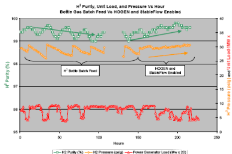
Figure2- Pressure stability vs. hydrogen purity
