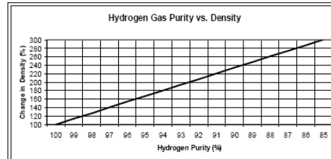
Figure 1- Relationship between hydrogen gas purity and gas density
