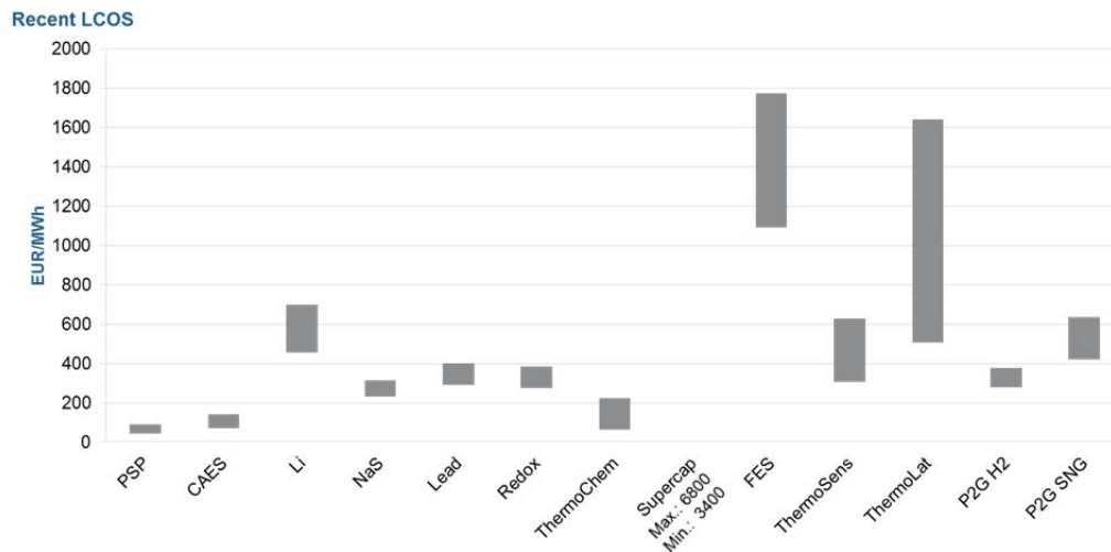
Figure 11: Levelised Cost of Storage co-located with PV in the 2015 study period (€_2014)
