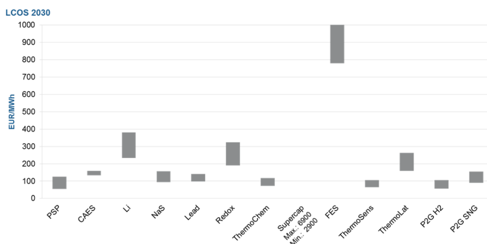
Figure 14: Levelised Cost of Storage co-located with wind in 2030 (€_2014)
