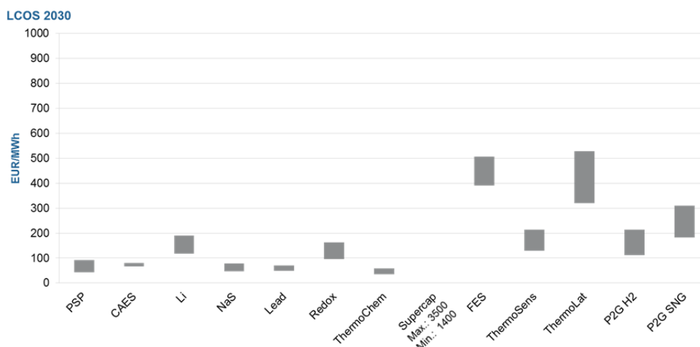
Figure 12: Levelised Cost of Storage co-located with PV in 2030 (€_2014)
