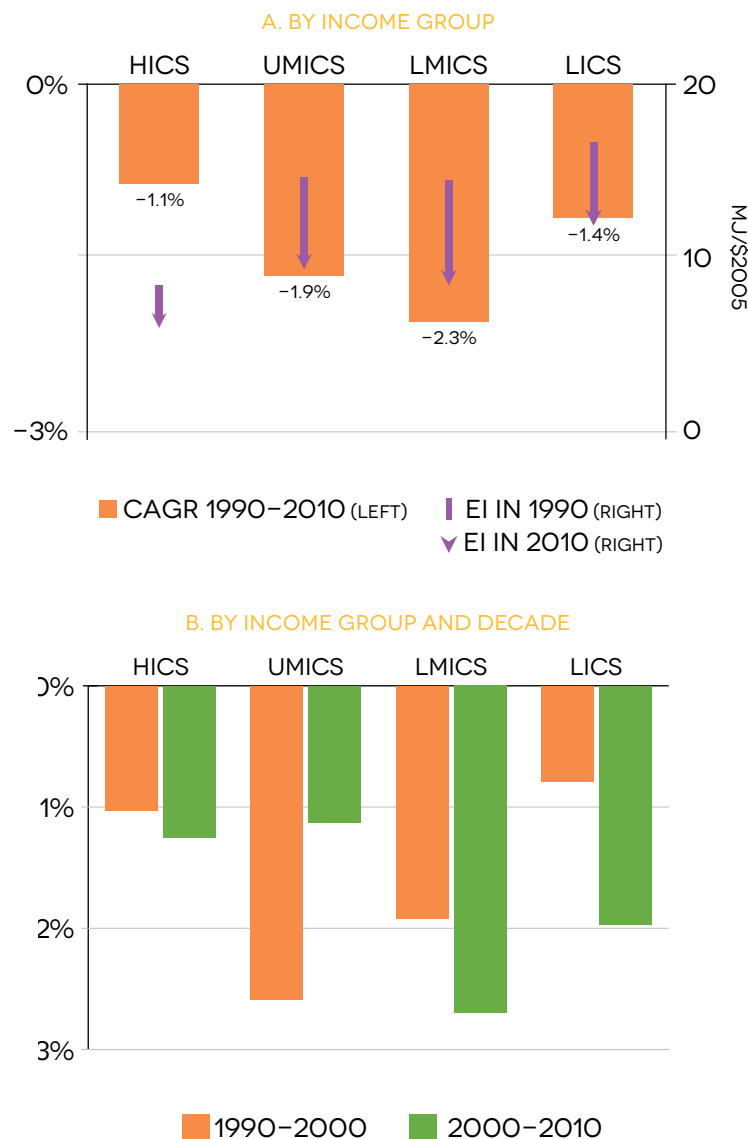
FIGURE 3.14 RATE OF IMPROVEMENT IN ENERGY INTENSITY AT PPP VS. ENERGY INTENSITY LEVELS IN 1990 AND 2010, BY COUNTRY INCOME GROUP AND DECADE
