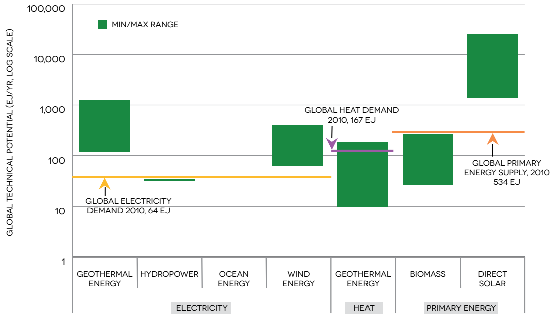
FIGURE 4.14 ESTIMATED GLOBAL TECHNICAL RE POTENTIAL
